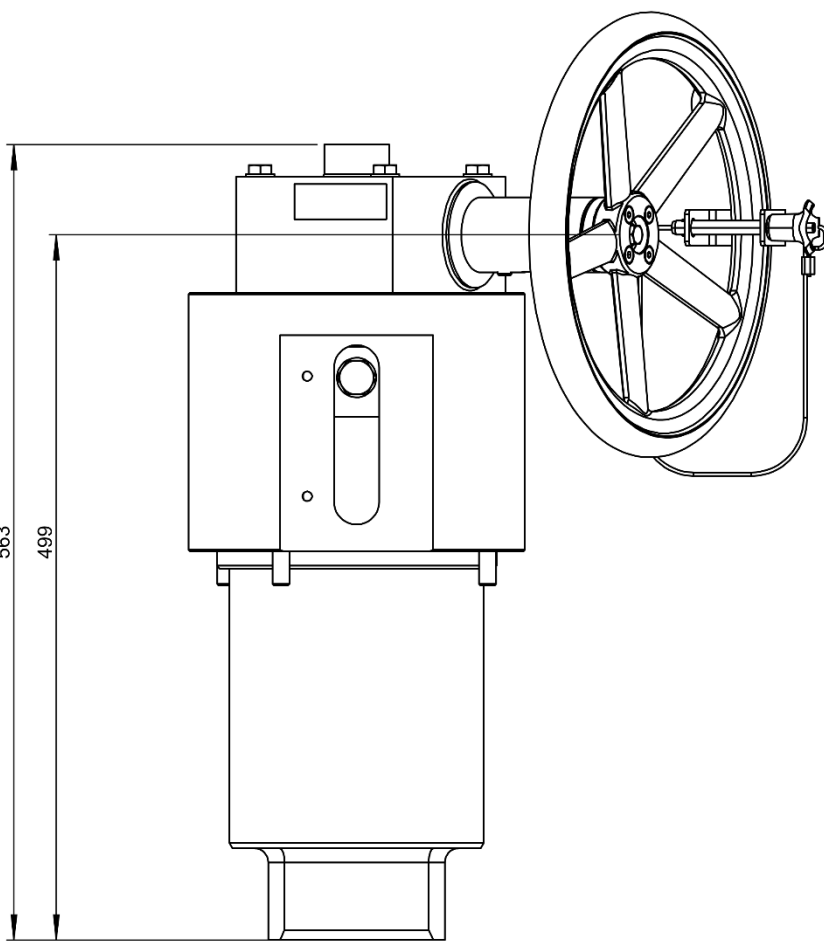
FRONT VIEW SCALE 1:5
